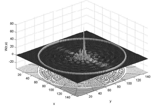
Fig. 6. Spatial structure W(r, \varphi) = \text{Im}(G_{\varphi\varphi}(r, a, \varphi)) in a cross-section 0 < r < 21 \mu\text{m} and 0 < \varphi < 2\pi of the microsphere with quasiperiodic stack for eigenfrequency f=436.09\text{THz} . A nanoemitter is placed at point a=900\text{nm} . Other parameters are as in Figure 2. One can see the confinement of field in the stack. Outer cycle indicates the external boundary R_{\text{ext}}=13.8\mu\text{m} of the quasiperiodic spherical stack.
