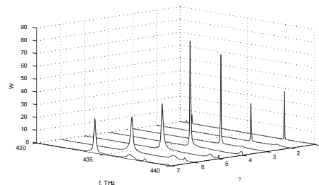
Fig. 5 . Spectrum of imaginary part of the Green's function W=G_{\varphi\varphi}(r,r) for r=900\text{nm} and 68 layers in stack (34 of 2-layer blocks F_9 ) for different values of parameter quasiperiodicity \gamma close to the golden mean value: 1) 0.55, 2) 0.58, 3) 0.6, 4) 0.618, 5) 0.63, 6) 0.65, 7) 0.68.
