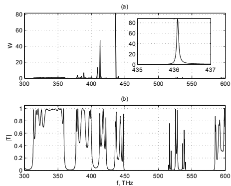
Fig. 4. (a) imaginary parts of tangential component of the Green's function W=G_{\varphi\varphi}(r,r) for r=900\text{nm} ; (b) Frequency spectrum of transmittance coefficient T for spherical quantum number m=9 . Microsphere is coated by quasiperiodic stack with N=68 (34 of 2-layers blocks, order Fibonacci F_9 ) for \gamma=0.618 . See details in text.
