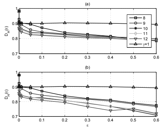
Fig. 7. Fractal (capacity) dimension D_{\{H\}}(\varepsilon) for Fibonacci stack F_{\{j\}} with j=8\div 12 and \gamma=0.5 . The last curve shows the periodic stack case with F_{\square\square} and \gamma=1 . (a) lossless stack; (b) dissipative stack.
